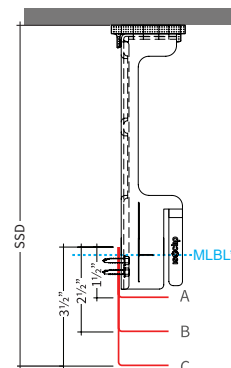
Plan Detail
