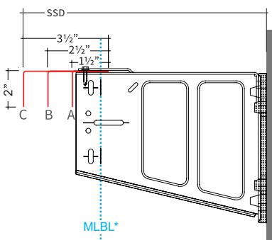
Section Detail
