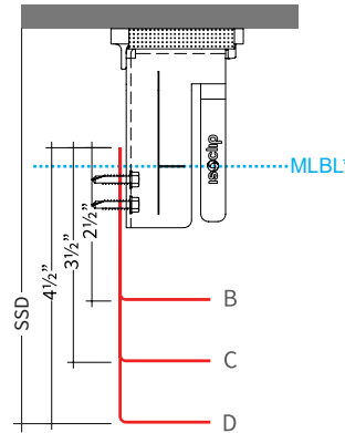
Plan Detail
