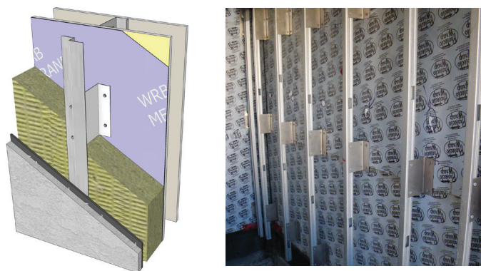
Intermittent stainless steel clips with vertical girts.
