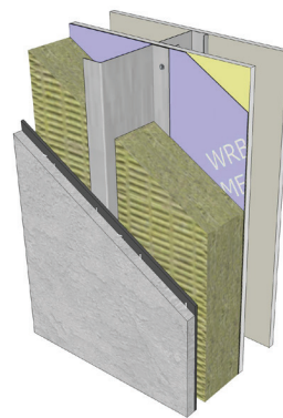
Vertical Z-girt over steel stud wall assembly. Girts are fastened to studs behind at every 16" o.c. resulting in significant thermal bridging through the exterior insulation.
