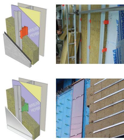
Fiberglass clips with vertical Z-girt attached with screw fasteners through the fiberglass clips into the back-up wall.
