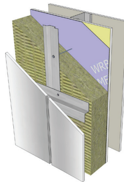
Long screws through horizontal metal hat tracks and rigid ROXUL COMFORTBOARD™ insulation on a commercial building project.
