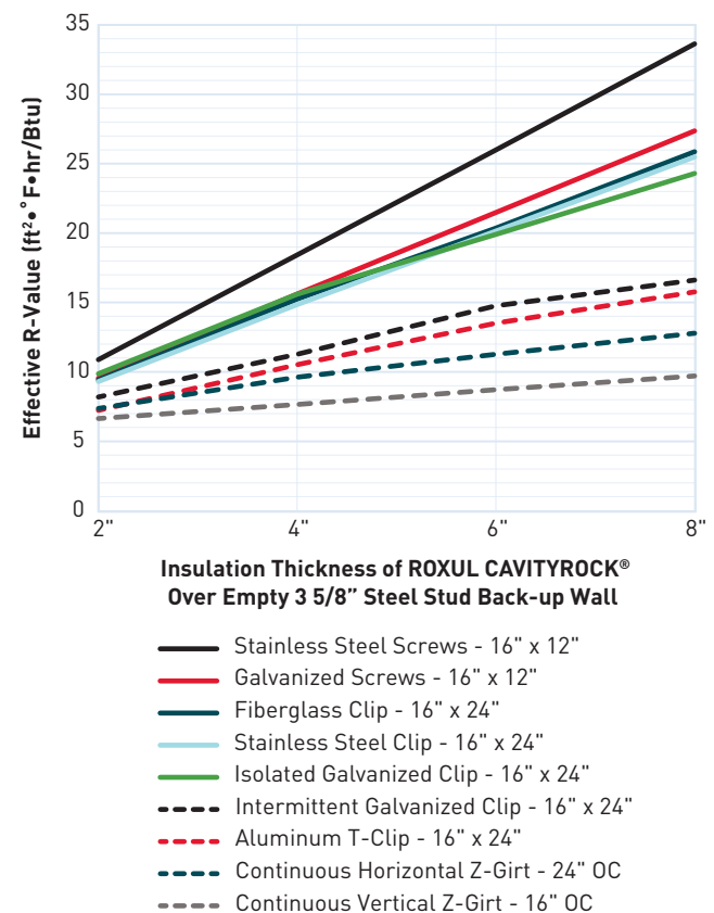
Uninsulated 3 5/8" steel stud wall with exterior insulation and cladding attachment system.
