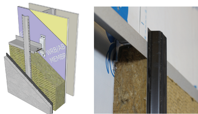
Aluminum T-clip with horizontal Z-girt and vertical hat-track for cladding attachment.
