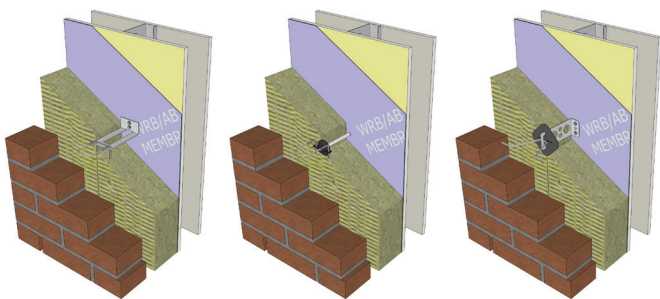
Examples of alternate masonry ties installed through ROXUL CAVITYROCK® insulation.
