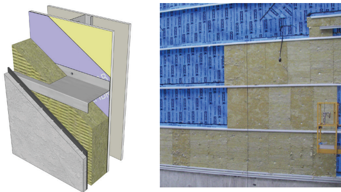
Horizontal Z-girts over a steel stud wall assembly. Girts are fastened every 36" here to reduce the thermal bridging.
