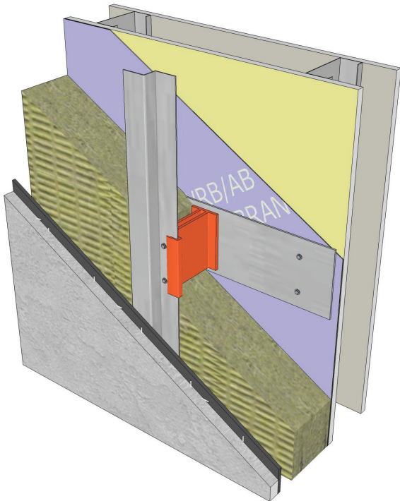
Example of the use of galvanized sheet steel strips to provide structural backer for cladding support clips away from studs.
