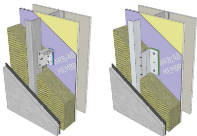
Additional examples of thermally isolated galvanized steel clips where low-conductivity pads are used to reduce the heat flow through each clip. Note that the best performance arises when the continuous girts attached to the clips are entirely outboard of the insulation and do not cut through it.
