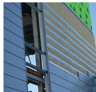
Long screws through horizontal metal hat tracks and rigid ROXUL COMFORTBOARD™ insulation on a commercial building project.
