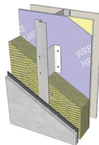
Intermittent galvanized steel clips with vertical girts.
