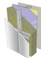
Long screws through rigid insulation utilizing continuous vertical strapping to create a truss cladding support system. Cladding attached to strapping on exterior of insulation.
