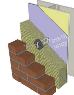
Masonry ties with semi-rigid insulation. The tie supports here provide only lateral resistance support, not gravity load (supported at the base of the veneer).
