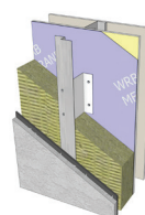
Discrete clip and rail type cladding support with semi-rigid insulation placed between clip supports inboard of the continuous vertical rail. Cladding attached back to vertical rails on exterior of insulation.
