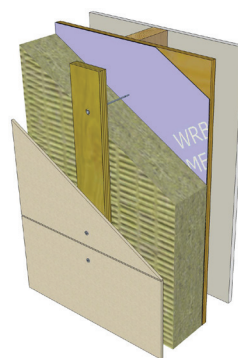
Long screws through vertical wood strapping and rigid ROXUL COMFORTBOARD™ insulation on a multi-family residential project.
