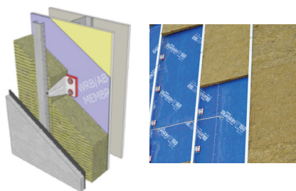
Thermally isolated galvanized steel clip attached to wall with screws through plastic isolation pad.
